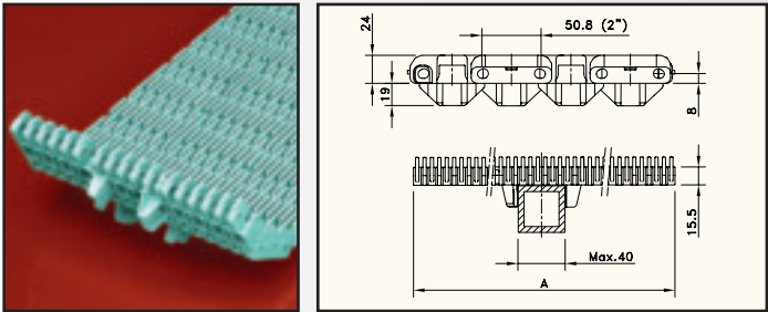
RAISED RIB 2000 BELT WITH POSITRACK IN THE CENTER OF THE BELT OR 1.5" OFFSET, DEPENDING ON THE WIDTH
