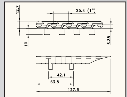
FLAT TOP 1005 HEAVY DUTY BELT WITH INTEGRATED FREEFLOW
